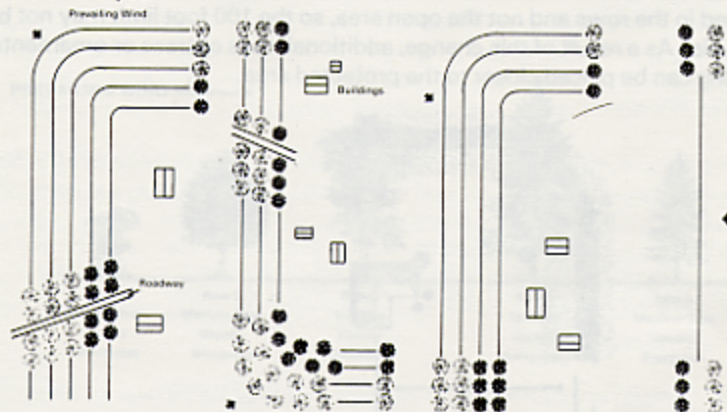
FIG. 6 Farmstead layout, prevailing wind direction and severity of snow drifting in your area are important factors to consider in windbreak planning. No set windbreak pattern can be prescribed. The sketches in this figure illustrate how windbreaks can be designed in different situations.
